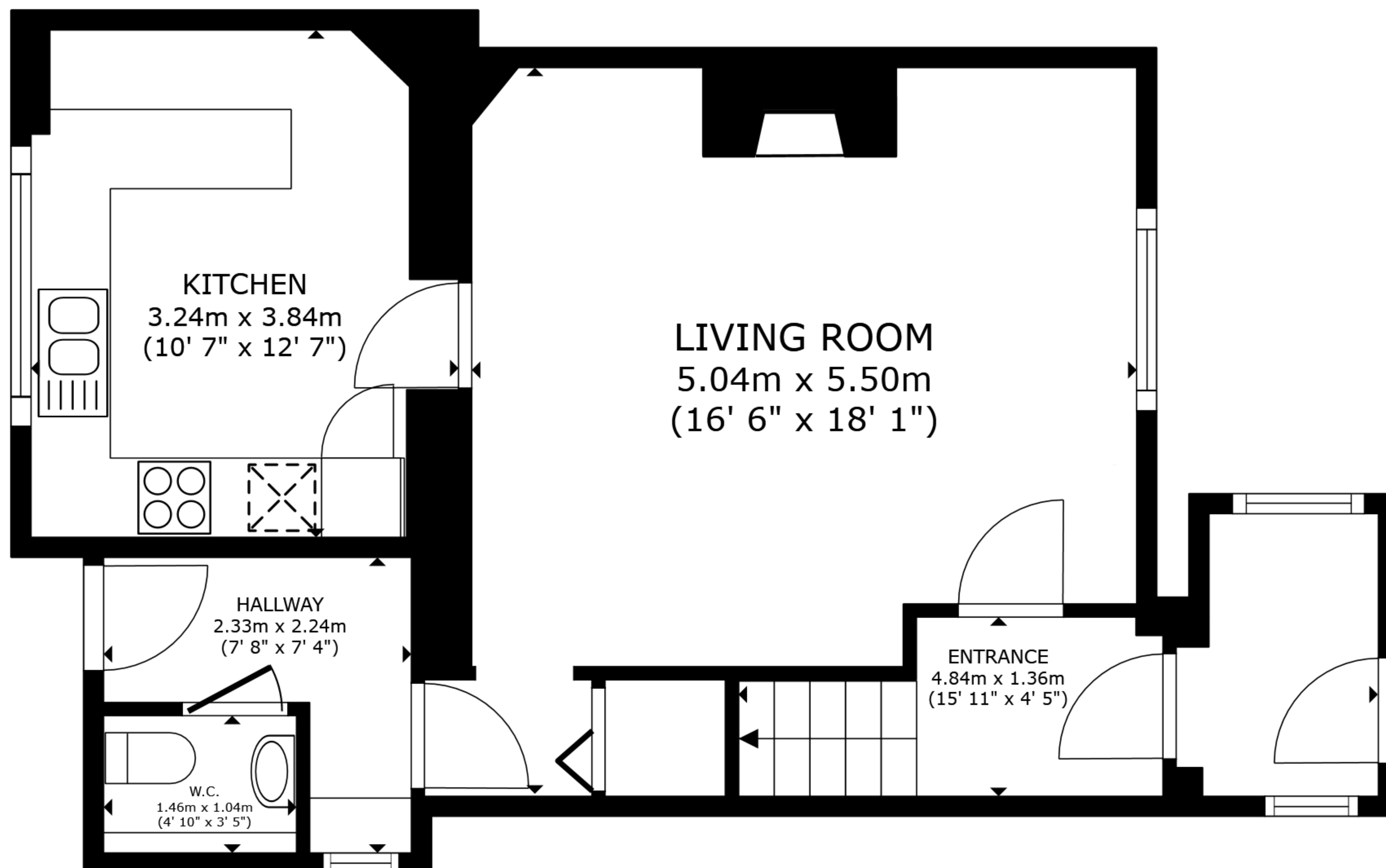
FLOOR 1
